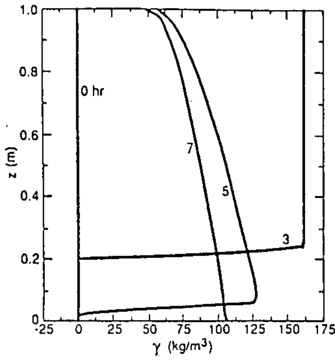
a. Bulk liquid density.
