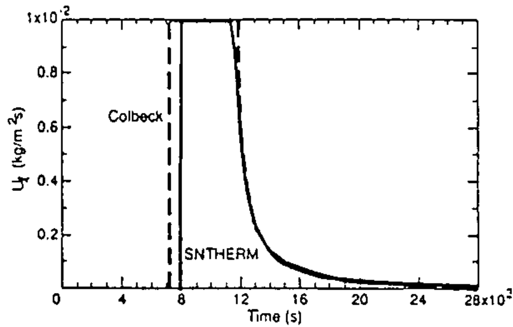
c. SNTHERM model predictions and computations of Colbeck (1976) for refrozen snow.
