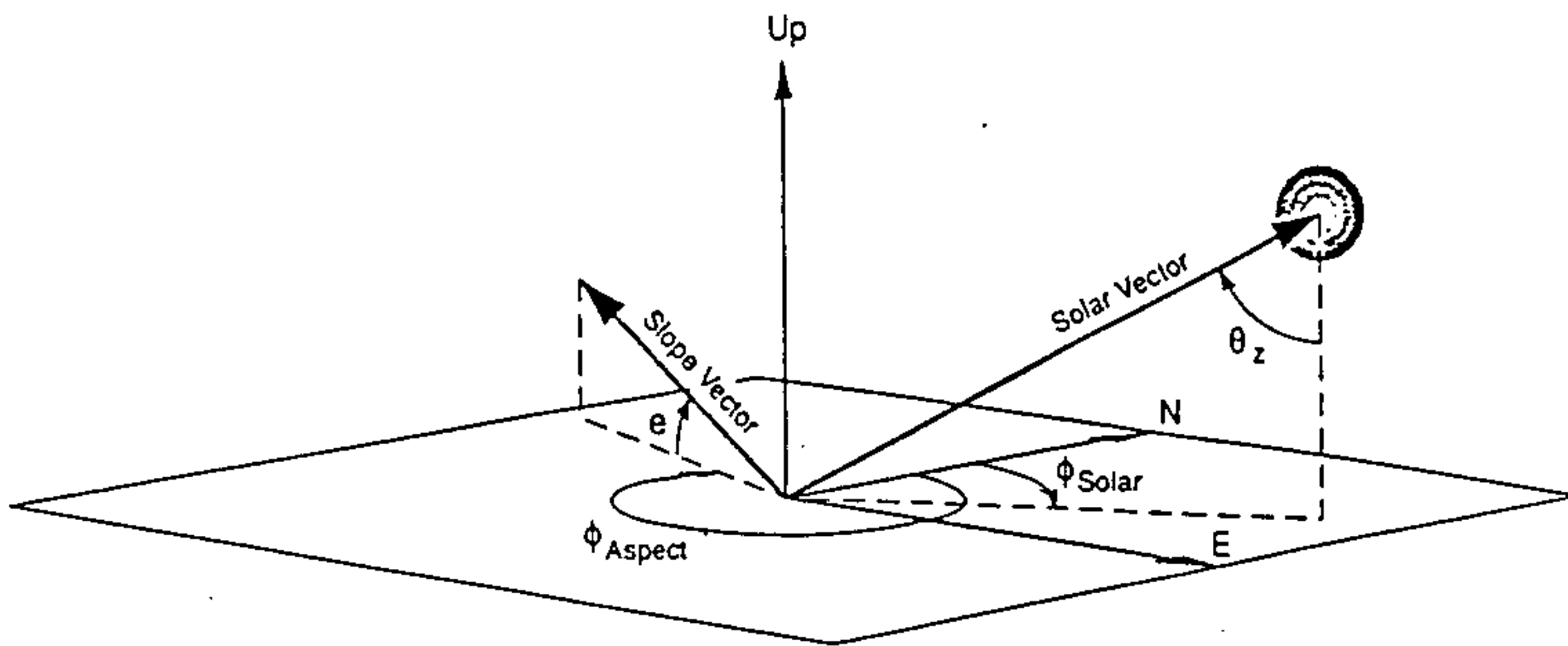
Figure 5. Geometry for radiation incident on a sloped surface.
