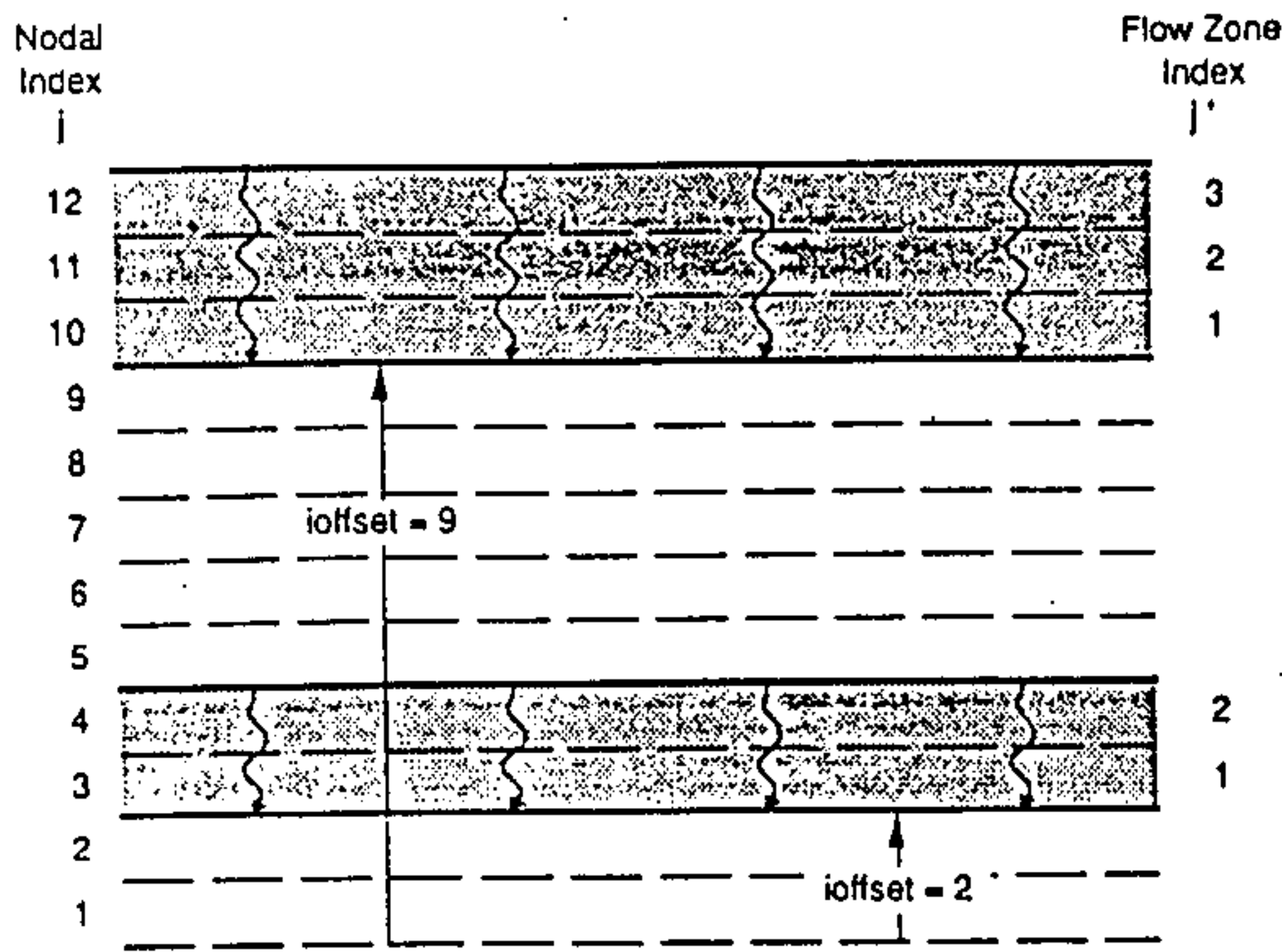
Figure 7. Diagram of flow zone system used in solution of fluid flow equations
