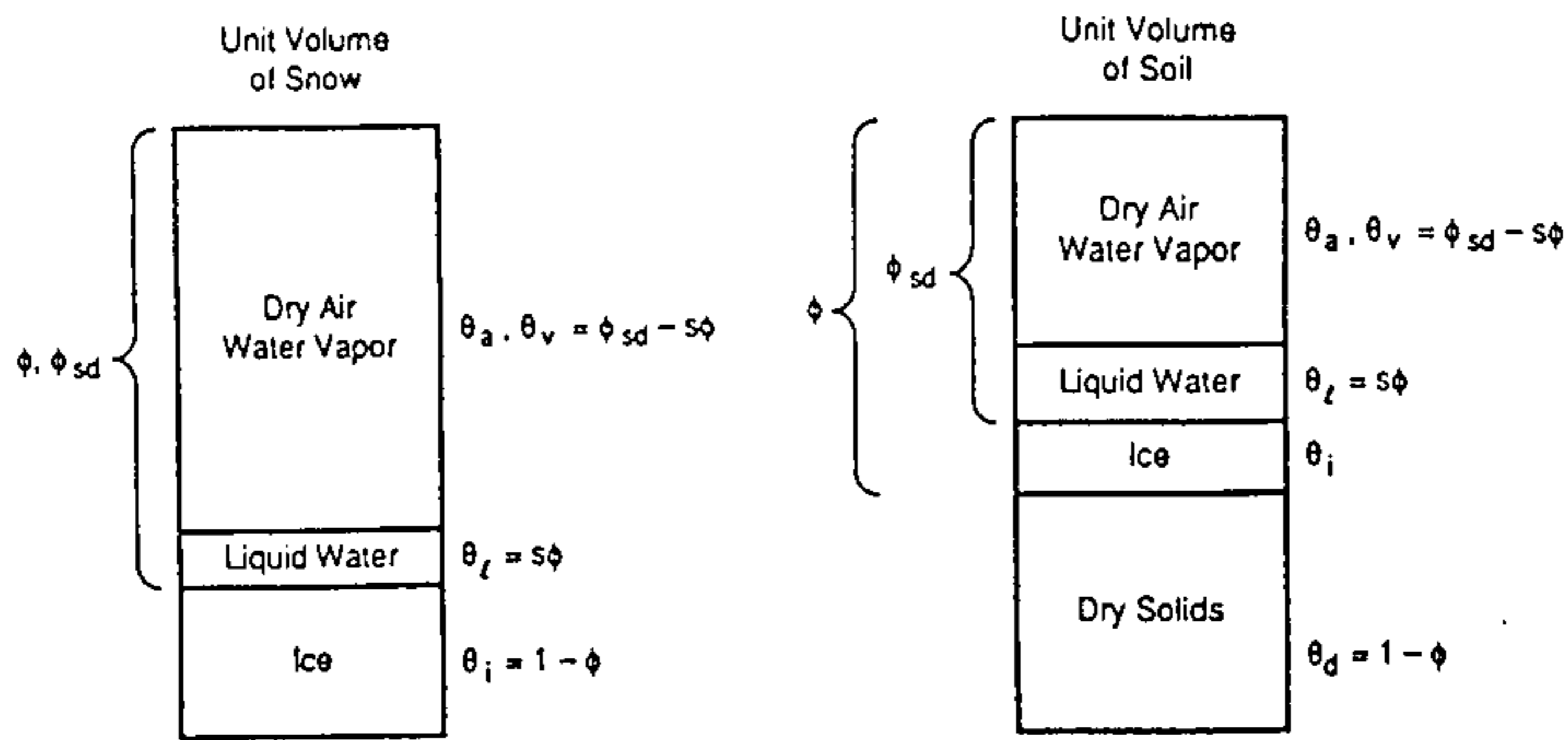
Figure 1. Fractional volume relationships in snow and soil. The air portion includes dry and wet (water vapor) components.
