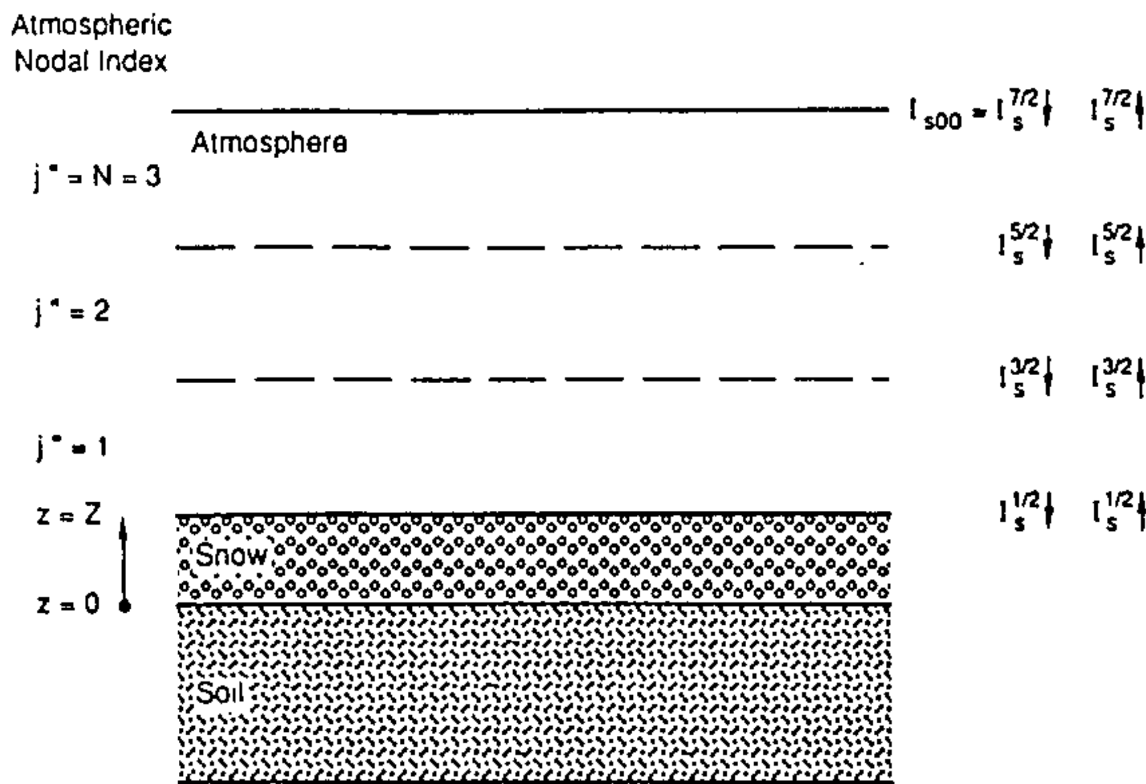
Figure 4. Conceptual geometry for a three-layer solar insolation model.
