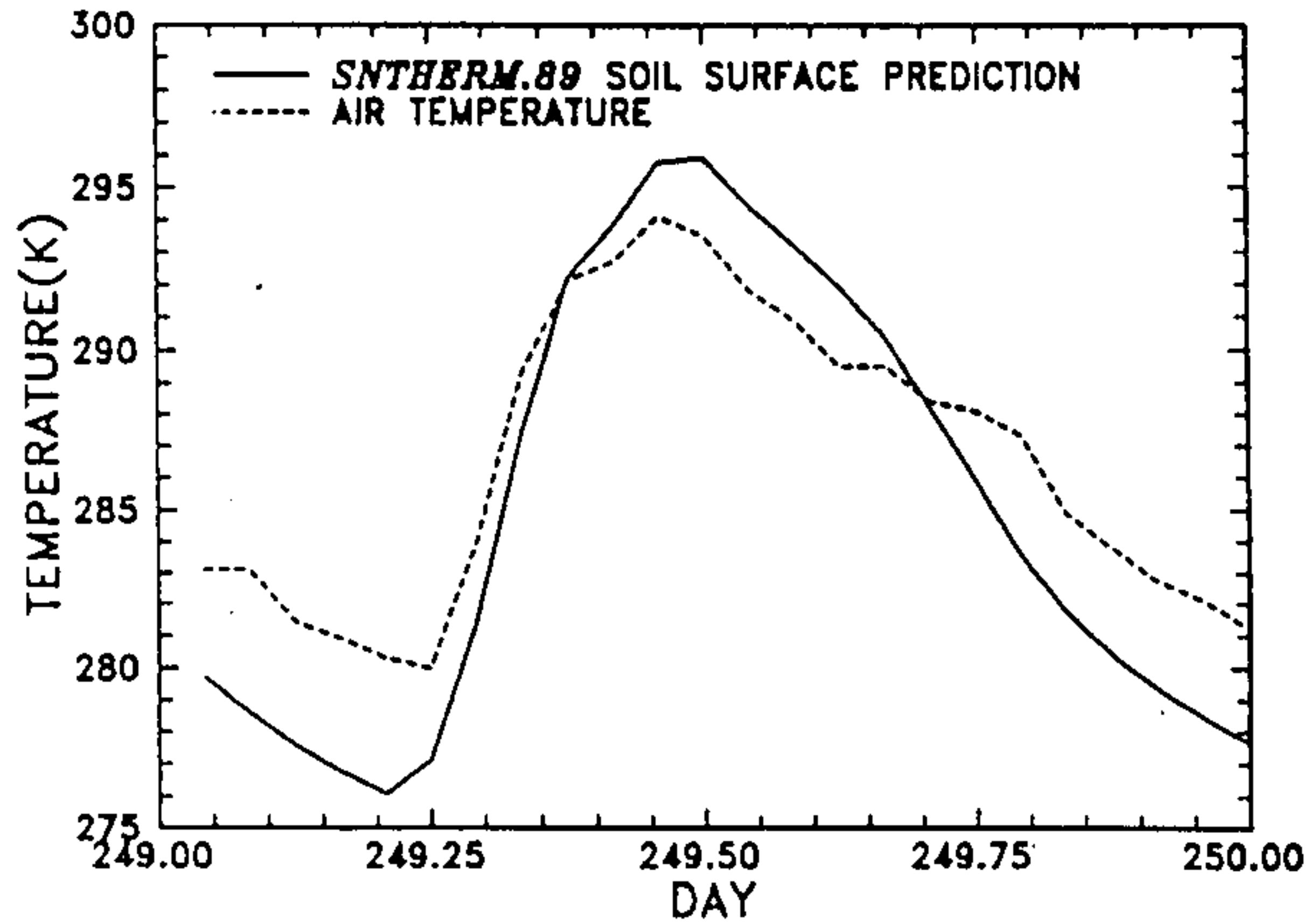
FIGURE 13. Predicted Soil Surface Temperature History and Air Temperature from Meteorological Data for Example Bare Soil Case
