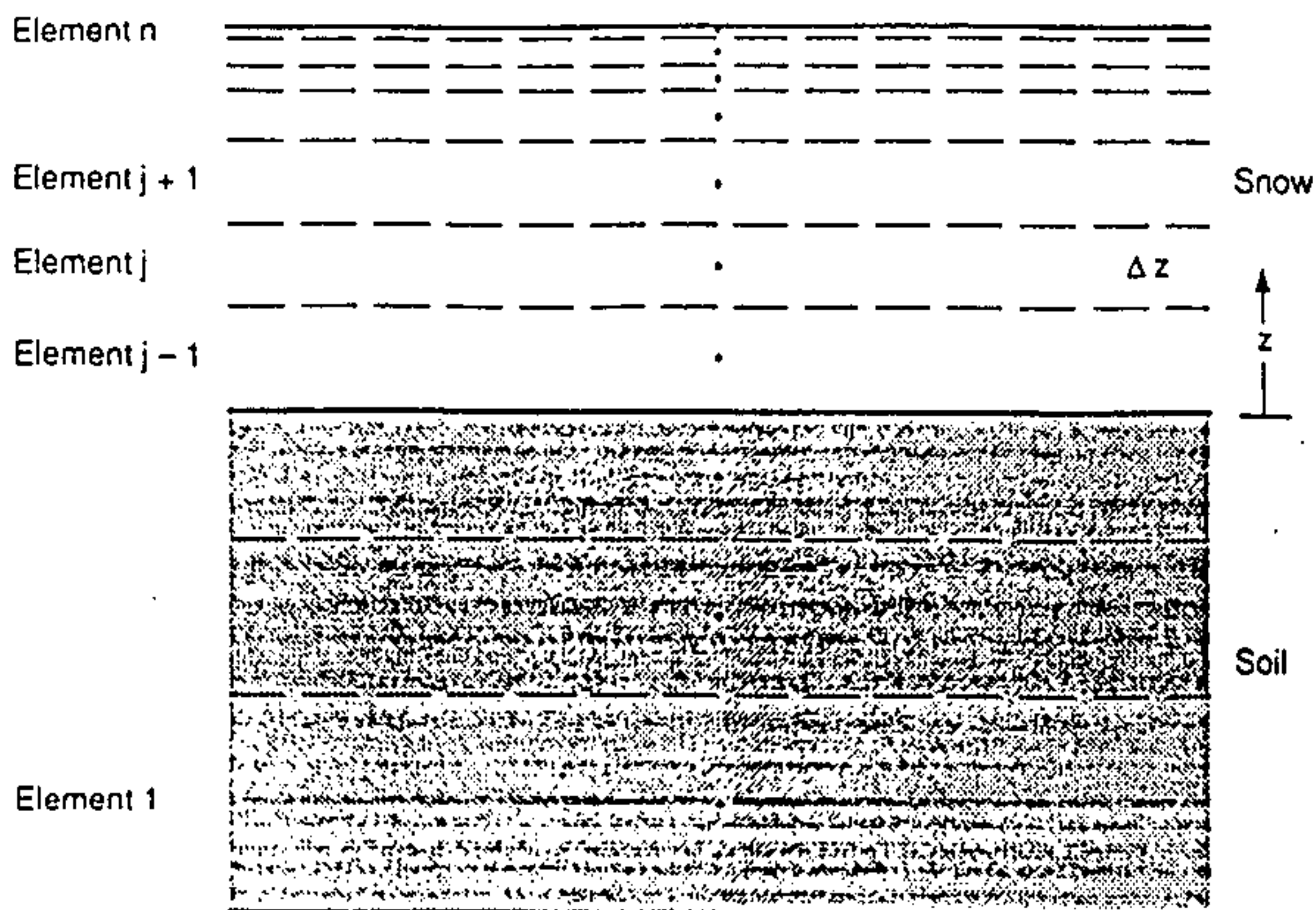
Figure 2. Finite-difference grid.
