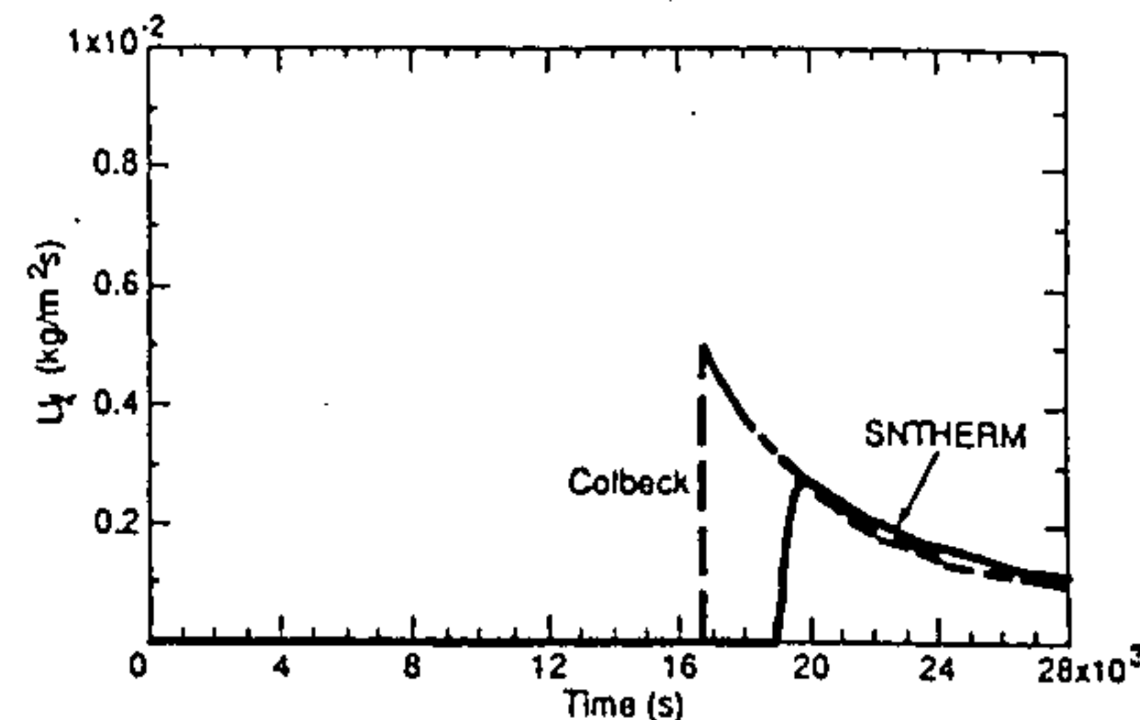
d. SNTHERM model predictions and computations of Colbeck (1976) for fresh snow.
