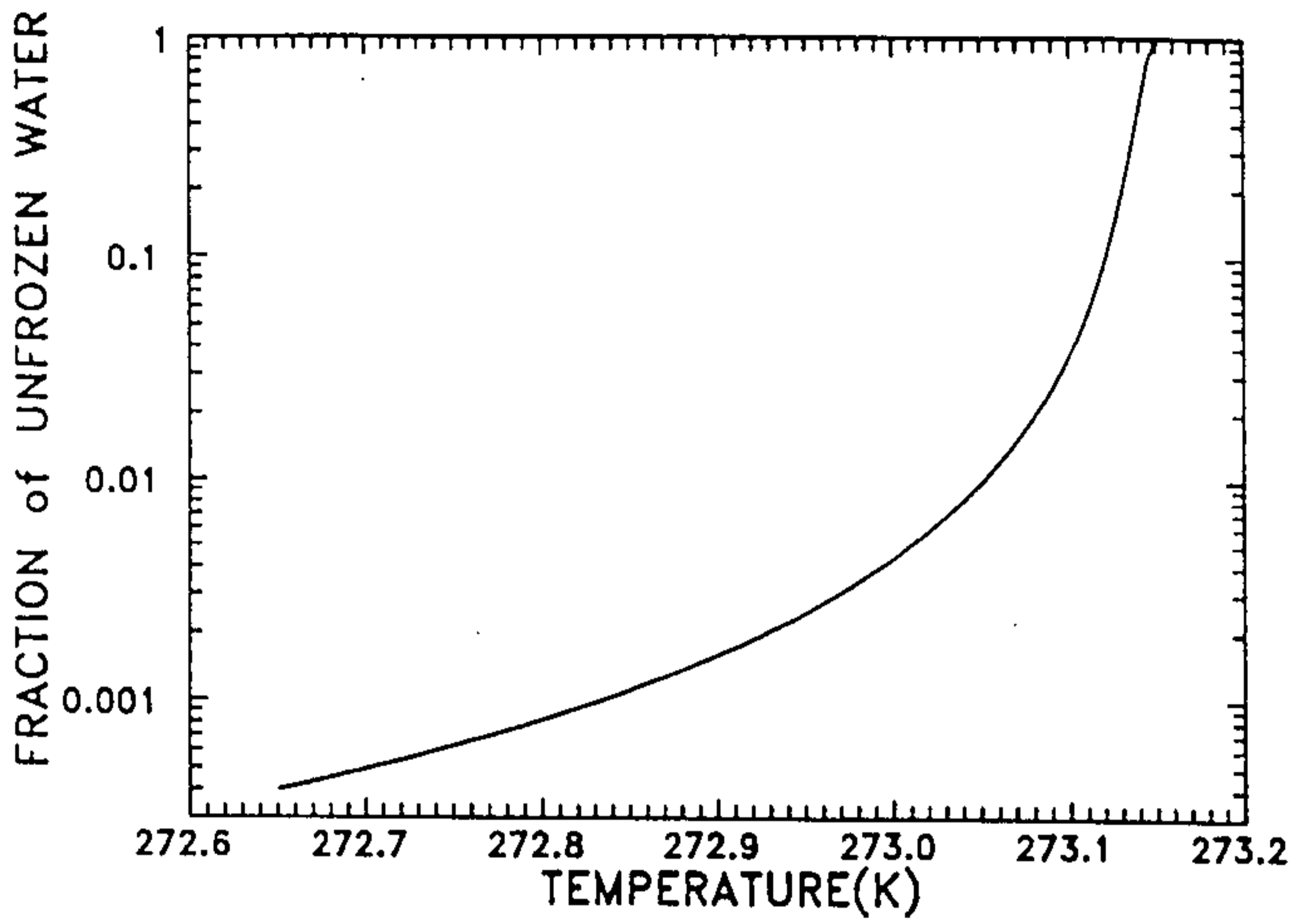
FIGURE 4. Freezing Curve to Aid Wet Snow Temperature Initialization
