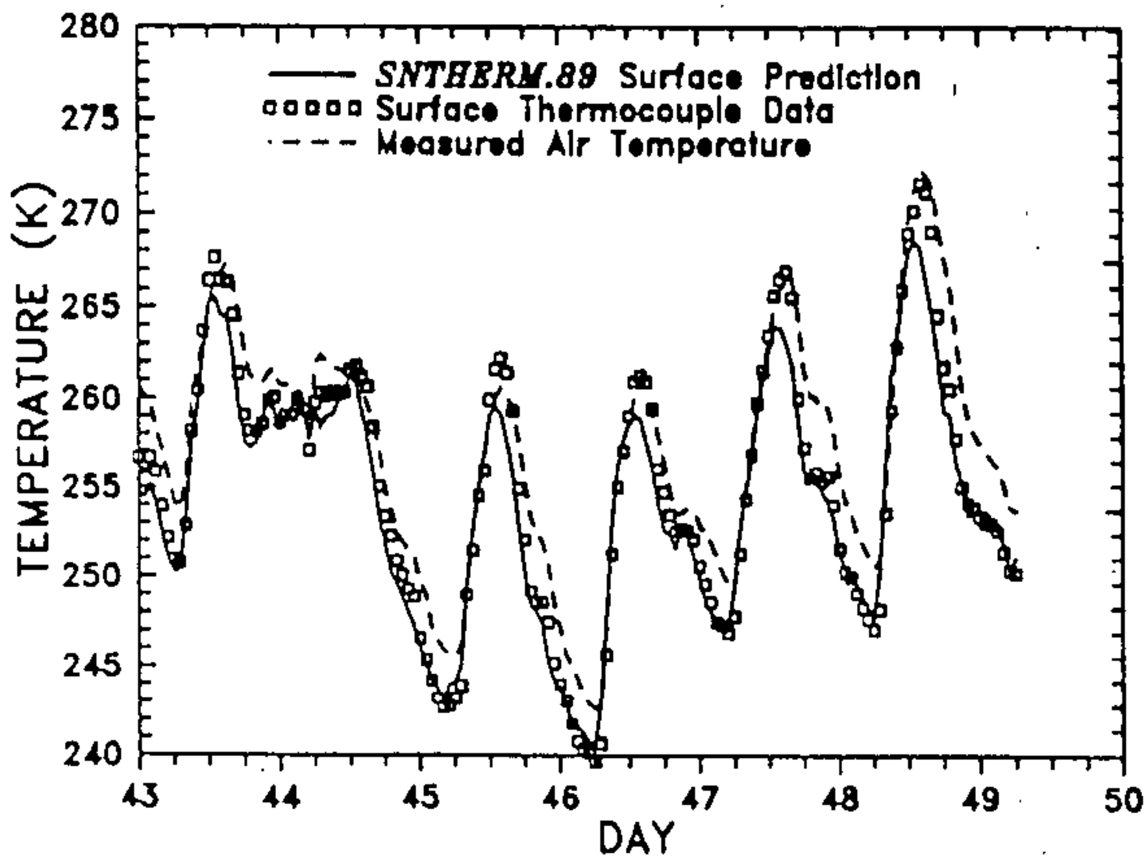
FIGURE 8. Predictions vs. Data. Surface Temperature Comparison. CRREL Data, Hanover, NH, Feb. 12-18, 1987
