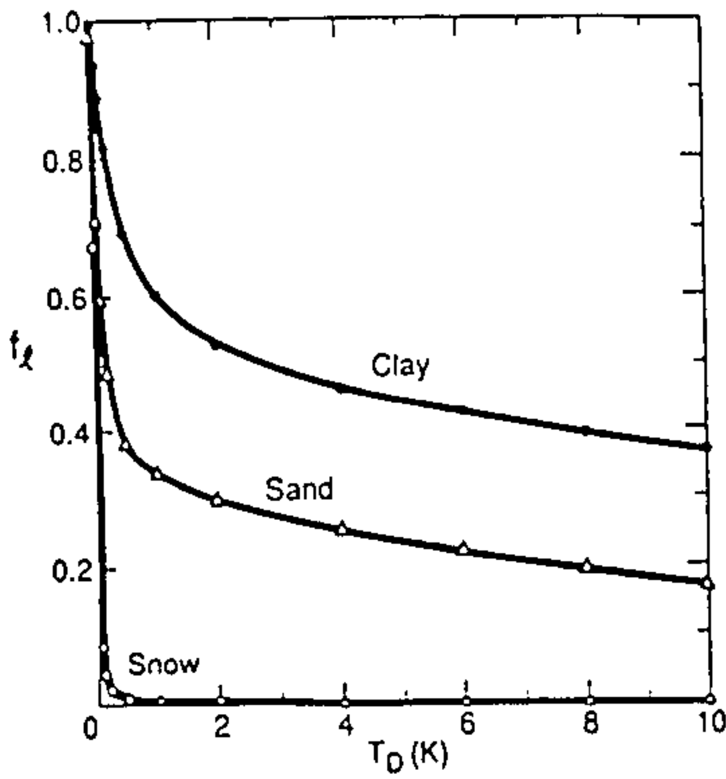
Figure 3. Mass liquid water fraction f_l predicted by eq 67.
