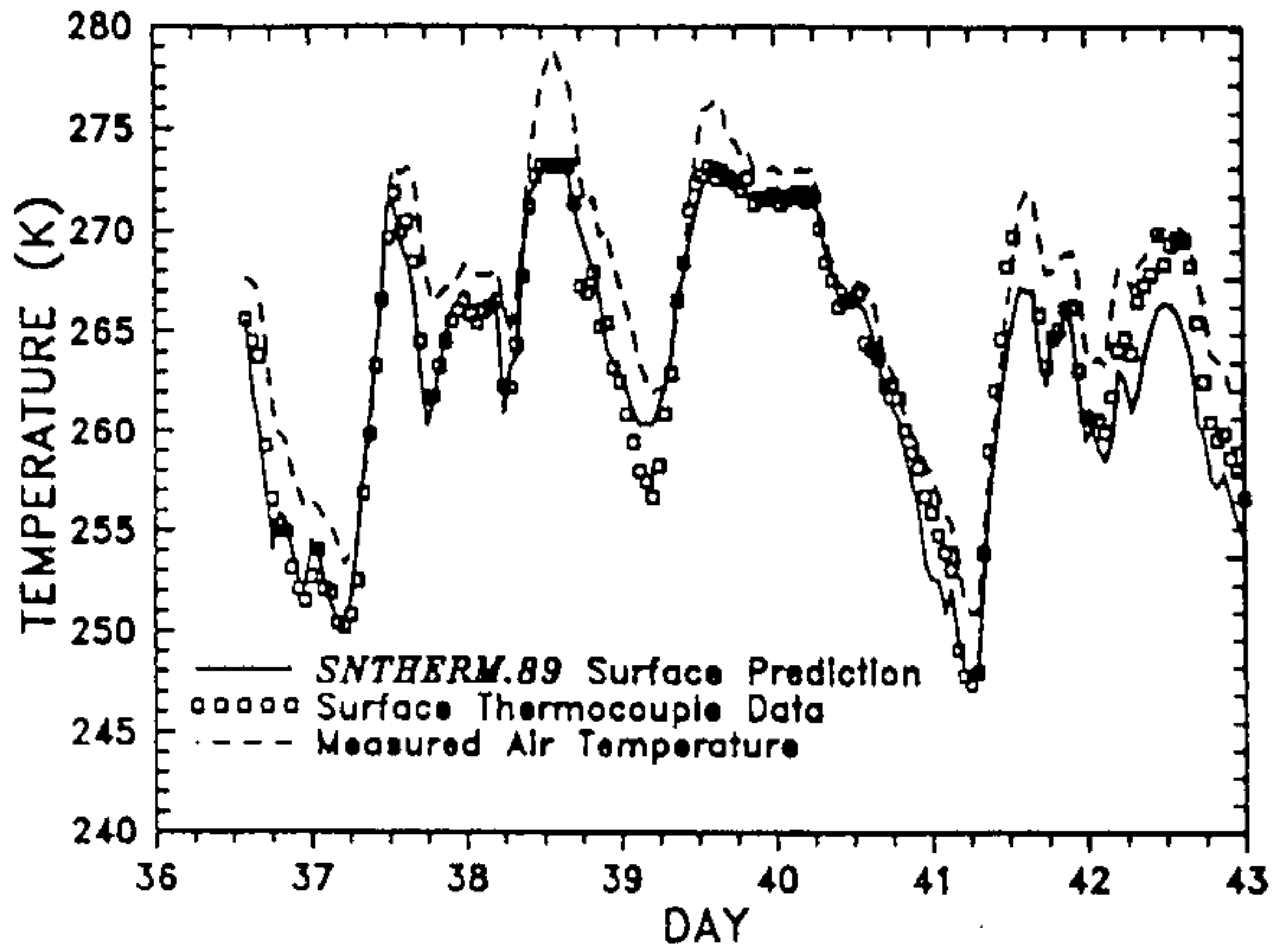
FIGURE 7. Predictions vs. Data. Surface Temperature Comparison. CRREL Data, Hanover, NH, Feb. 5-11, 1987
