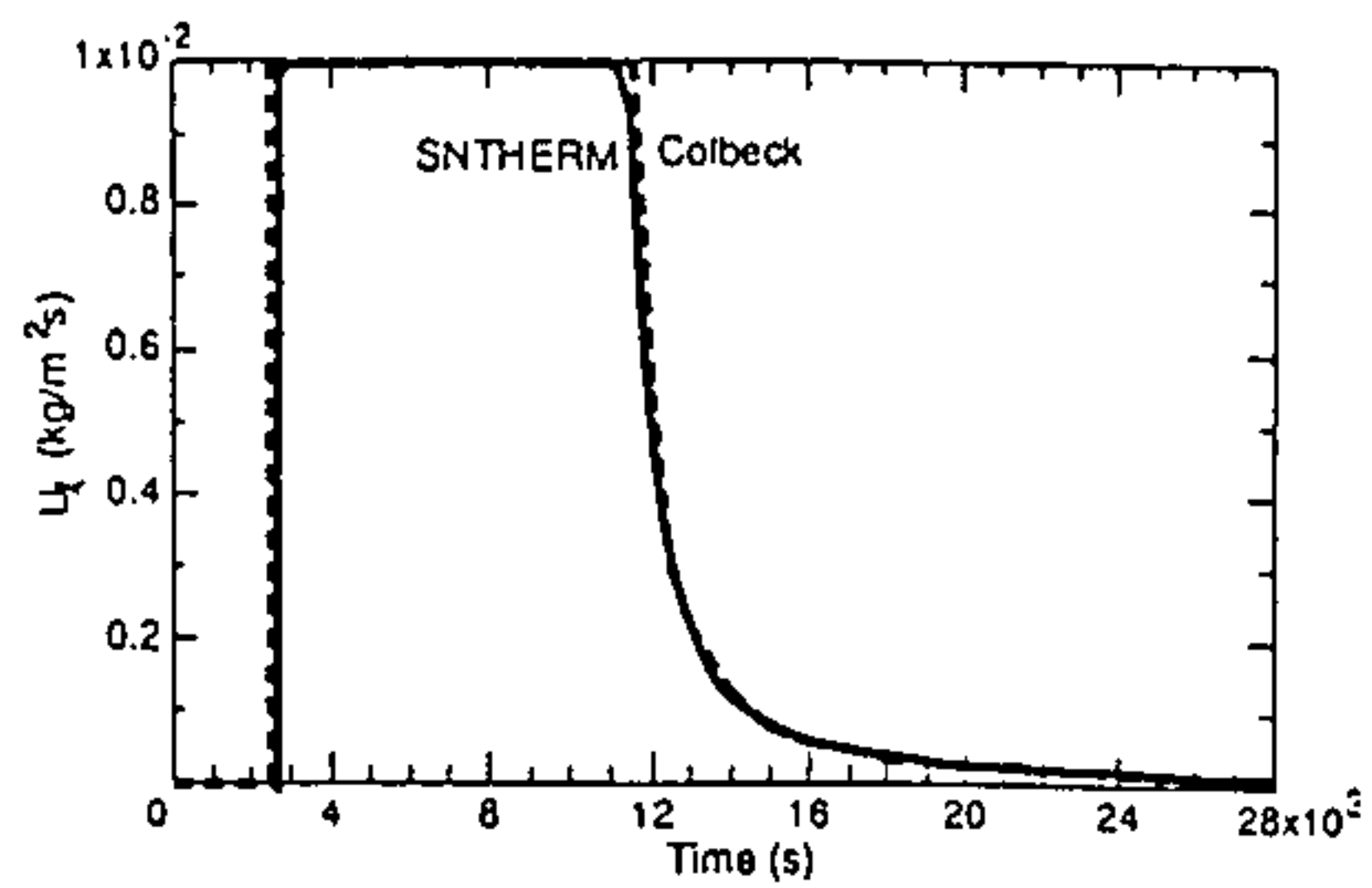
b. SNTHERM model predictions and computations of Colbeck (1976) for ripe snow.
